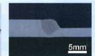
·Welding electric current:300A ·Welding voltage:22V ·Sheet thickness:3.2mm ·Wire diameter:φ1.2mm ·Welding speed:150cm/min ·Wire feeding speed:11.0m/min ·Protrusion:15mm
