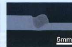
·Welding electric current:300A ·Welding voltage:22V ·Sheet thickness:3.2mm ·Wire diameter:φ1.2mm ·Welding speed:150cm/min ·Wire feeding speed:11.0m/min ·Protrusion:15mm
