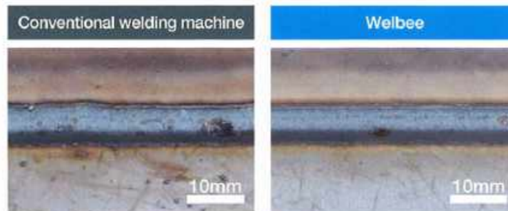
·Welding electric current:230A ·Welding voltage:23.5V ·Shield gas:80%Ar+20%CO 2 ·Welding base material:Galvanized sheet iron:45g/m 2 , 2.3mm ·Welding speed:100cm/min ·Wire diameter:φ1.2mm ·Welded joint:Overlapped fillet welding
