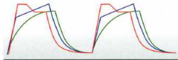
— MAG pulse waveform for soft steels (WB-P500L) — MIG pulse waveform for stainless steels — MIG pulse waveform for aluminum
