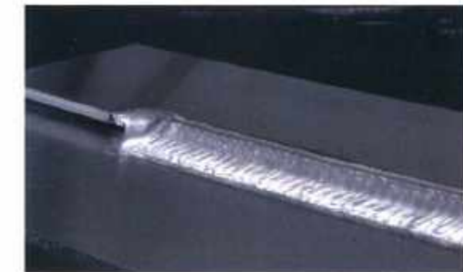
·Welding electric current:120A ·Welding voltage:16V ·Sheet thickness:3.0mm ·Wire diameter:φ1.2mm ·Welding speed:50cm/min ·Wave frequency:2.5Hz
